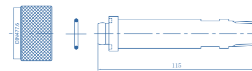
Hand tight nut & nipple (Example: VCC-C-HNN-DIN477.6)
