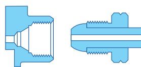
CGA 590 .965" -14 NGO LH INT.
