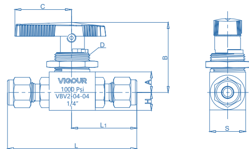
Straight-through type
