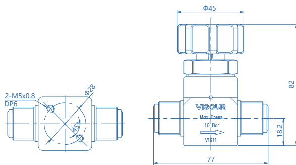
1/2 manual actuator (VFS fitting male)
